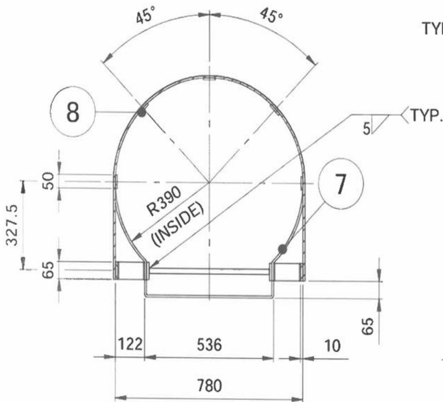
SECTION B-B
